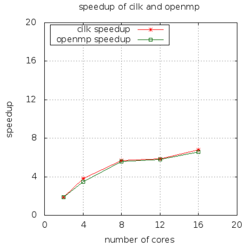
Figure 5.5: Naive Matrix Multiplication : n = 4096
