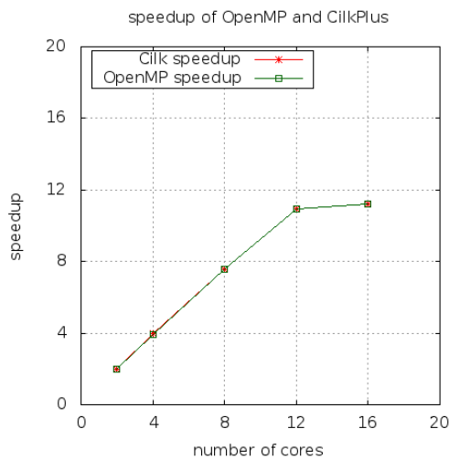
Figure 5.16: Sparse LU matrix factorization.
