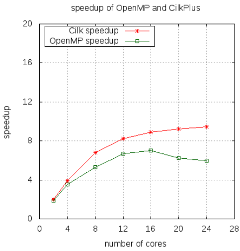
Figure 5.15: Mergesort (BOTS).
