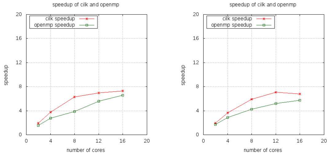
(a) Quick Sort: n = 2 \cdot 10^8
